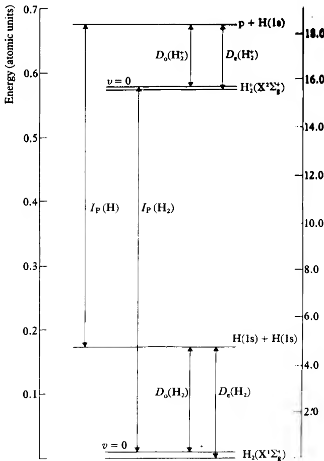
9.14 Relationships between the ground state energies of H_2 , H_2^+ and H . The chemical dissociation energies and spectroscopic dissociation energies denoted by D_0 and D_e , respectively, differ by the zero-point vibrational energy \frac{1}{2}\hbar\omega_0 . The ionisation potentials of the hydrogen atom and hydrogen molecule are denoted by I_P(H) and I_P(H_2) .
